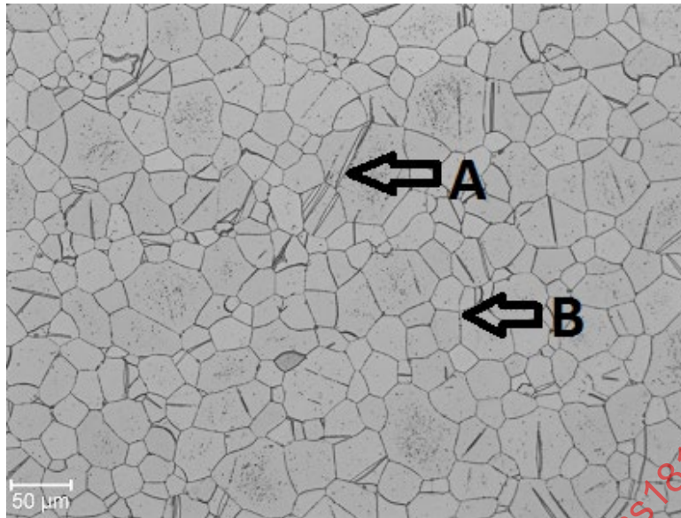
ETCHANT: 2%HF 200X ALLOY COMMERCIALLY PURE (CP). TWIN "A" IN EQUIAXED ALPHA "B"
