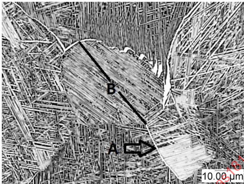
ETCHANT: KROLL'S 600X ALLOY 6Al-2Sn-4Zr-6Mo. GRAIN BOUNDARY ALPHA "A" SURROUNDING PRIOR BETA GRAINS "B".
