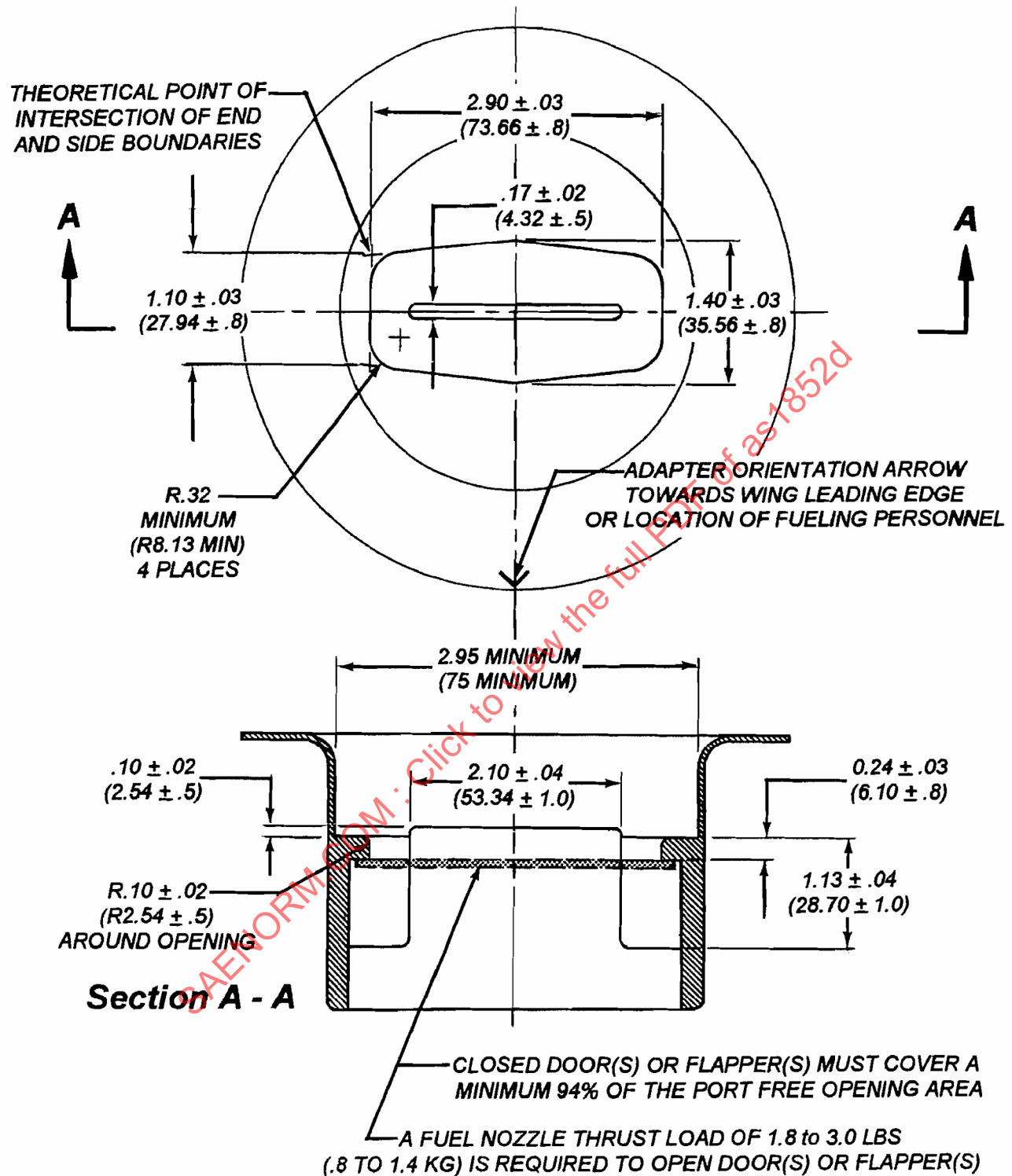
FIGURE 1 - Turbine Fuel Service Port
