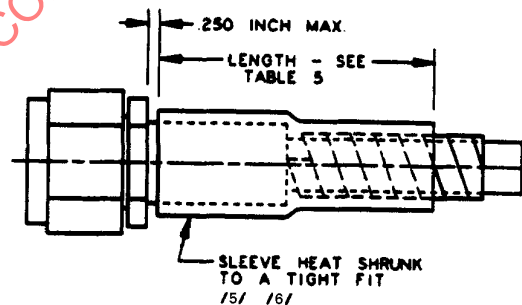
FIGURE 3 - ABRASION SLEEVE RETENTION
