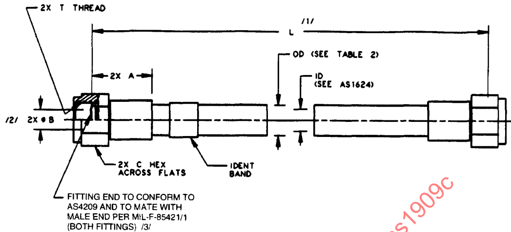
FIGURE 1 - HOSE AND FITTING DIMENSIONS
