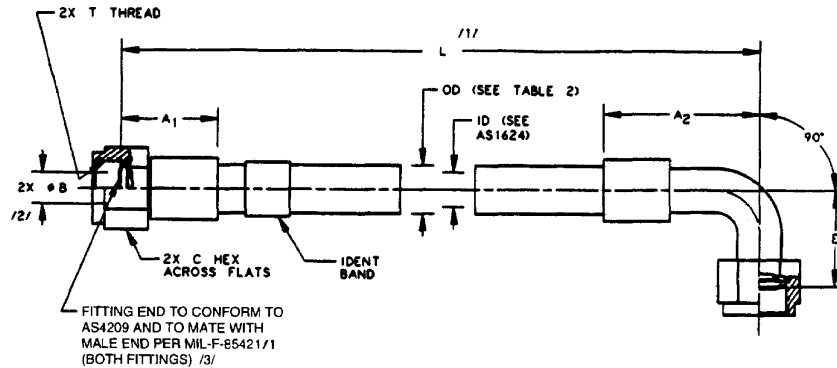
FIGURE 1 - HOSE AND FITTING DIMENSIONS
