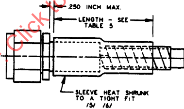
FIGURE 3 - ABRASION SLEEVE RETENTION
