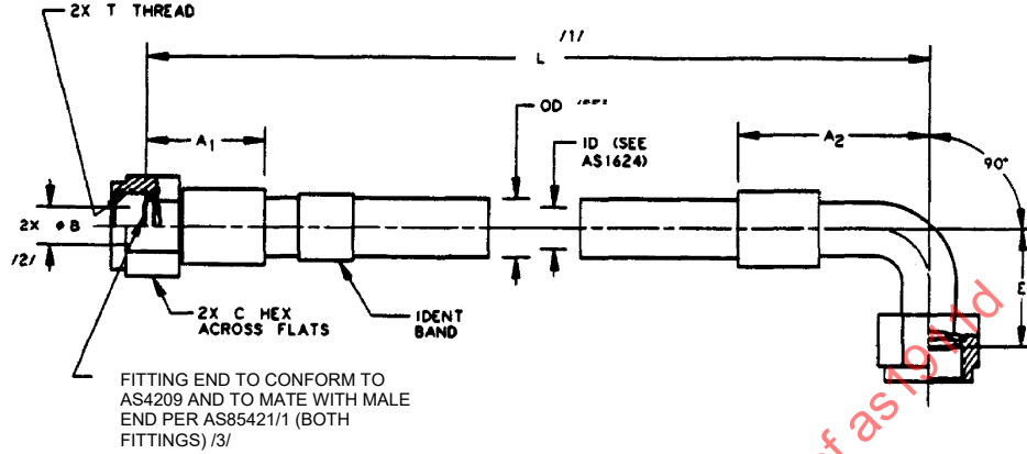
FIGURE 1 - HOSE AND FITTING DIMENSIONS
