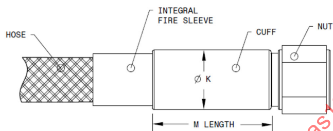
FIGURE 5 - INTEGRAL FIRESLEEVE CUFF DIMENSIONS - SEE TABLE 7 /27/
