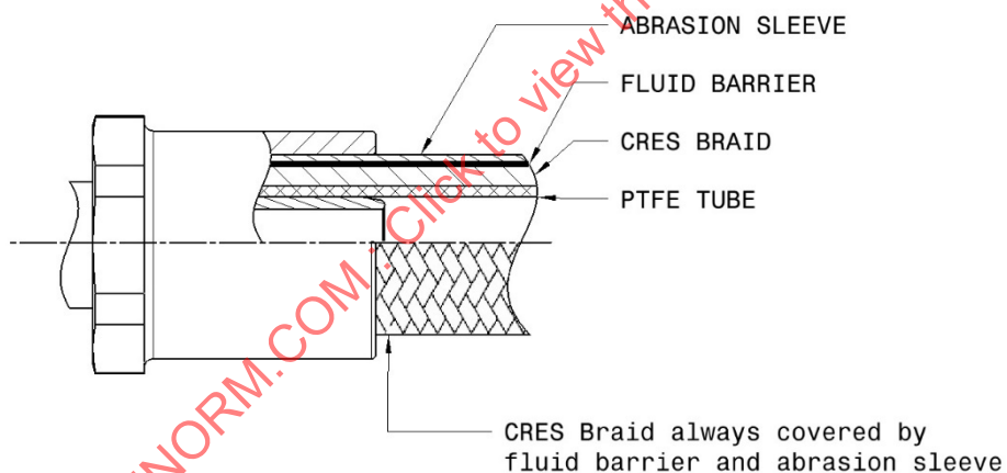
FIGURE 6 - FITTING CAPTURED INTEGRAL ABRASION SLEEVE WITH FLUID BARRIER /28/
