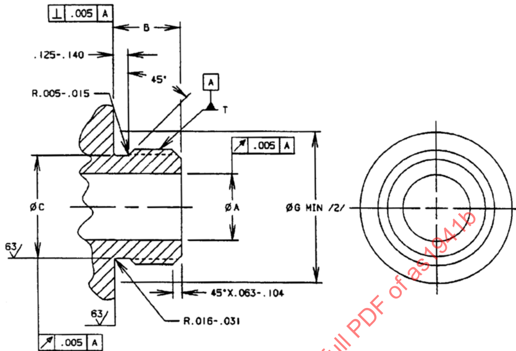
FIGURE 1 - FITTING END
