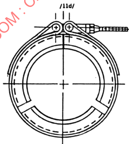
FIGURE 5 - INCORRECT INSTALLATION RETAINERS OR BAND TOUCHING
