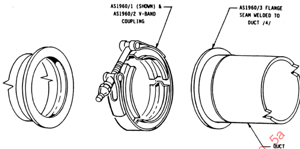
FIGURE 1 - EXPLODED VIEW OF JOINT COMPONENTS
