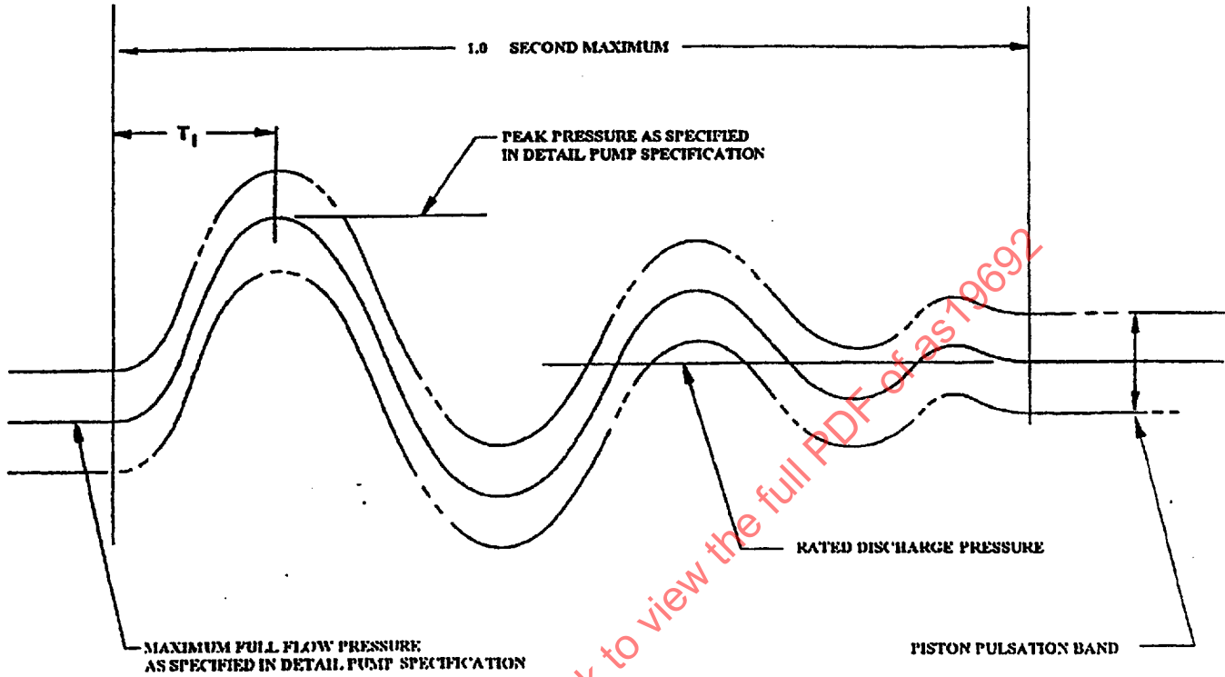
FIGURE 3. Typical pressure transient full flow to zero flow
