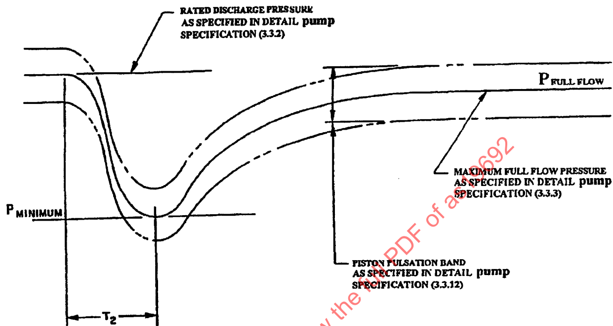
FIGURE 4. Typical pressure transient zero flow to full flow
