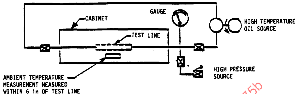
FIGURE 2 - Typical Setup for Thermal Shock Testing
