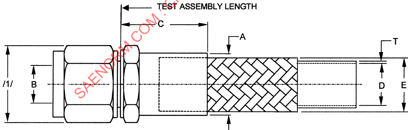
FIGURE 1 - Hose and Fitting Dimensions
