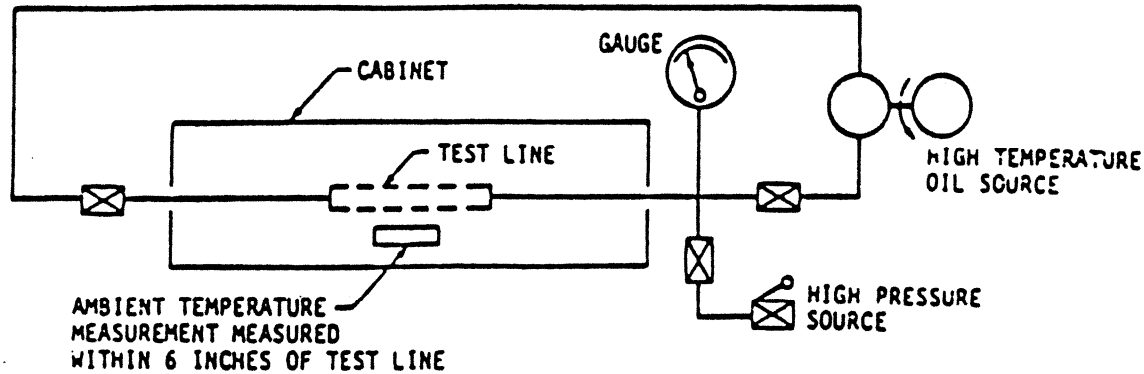
FIGURE 2 - TYPICAL SETUP FOR THERMAL SHOCK TESTING
