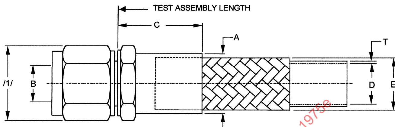
FIGURE 1 - HOSE AND FITTING DIMENSIONS
