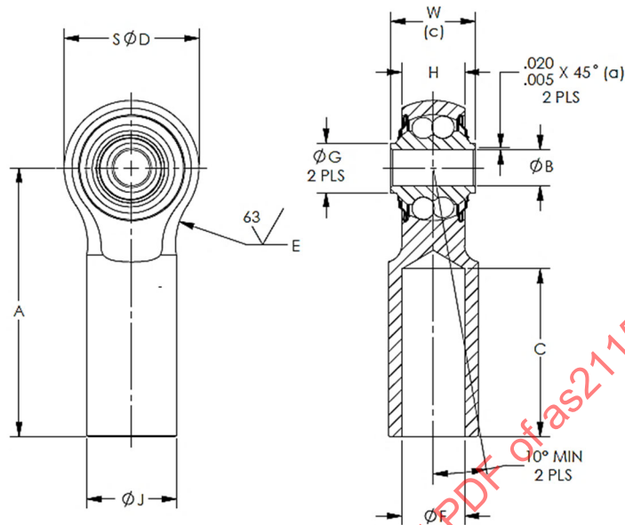
FIGURE 1 - PART CONFIGURATION
