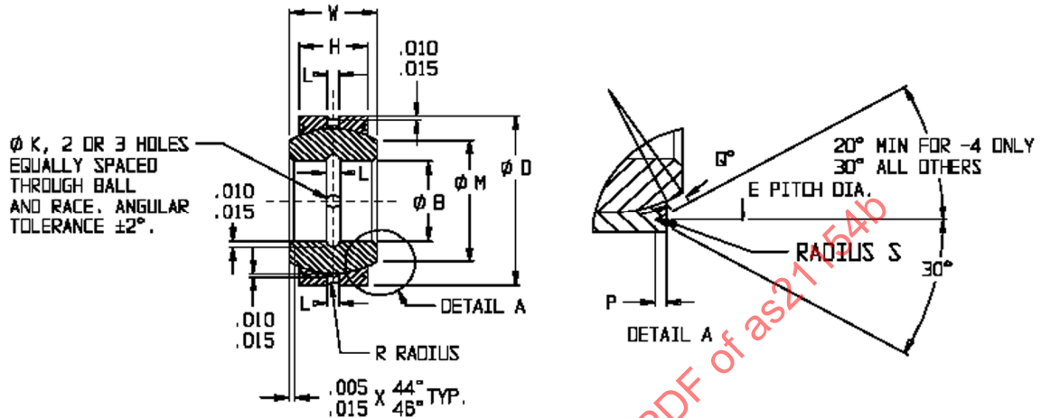
FIGURE 1 – PART CONFIGURATION
