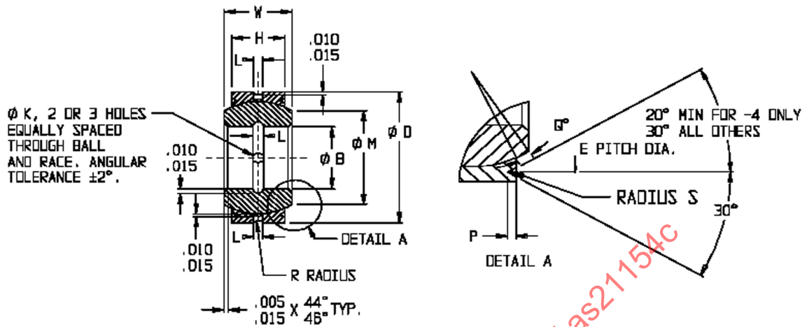
FIGURE 1 – PART CONFIGURATION
