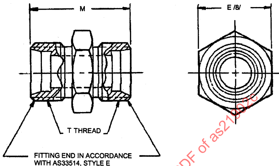
FIGURE 1 - UNION, FLARELESS TUBE
