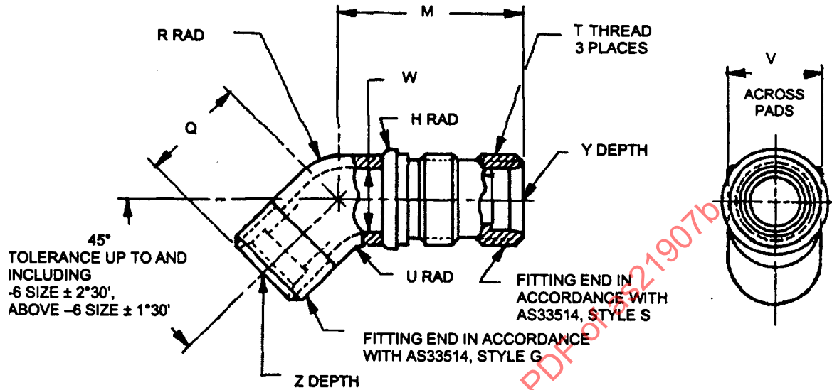
FIGURE 1 - ELBOW, BULKHEAD UNIVERSAL, 45°, FLARELESS TUBE
