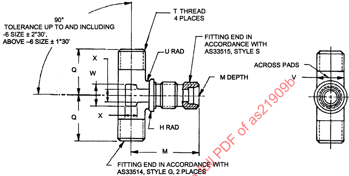
FIGURE 1 - TEE, BULKHEAD AND UNIVERSAL, FLARELESS TUBE
