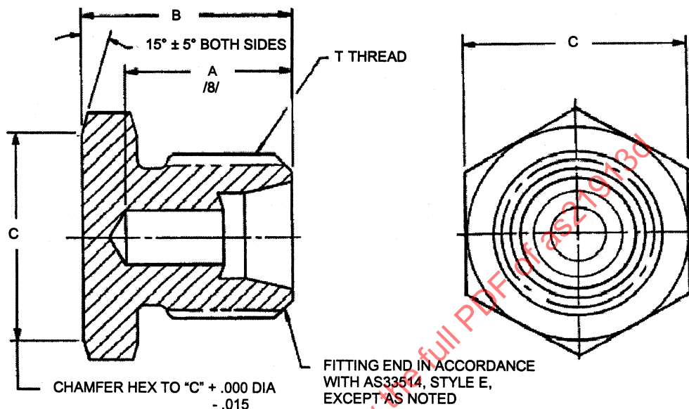
FIGURE 1 - PLUG, FLARELESS TUBE
