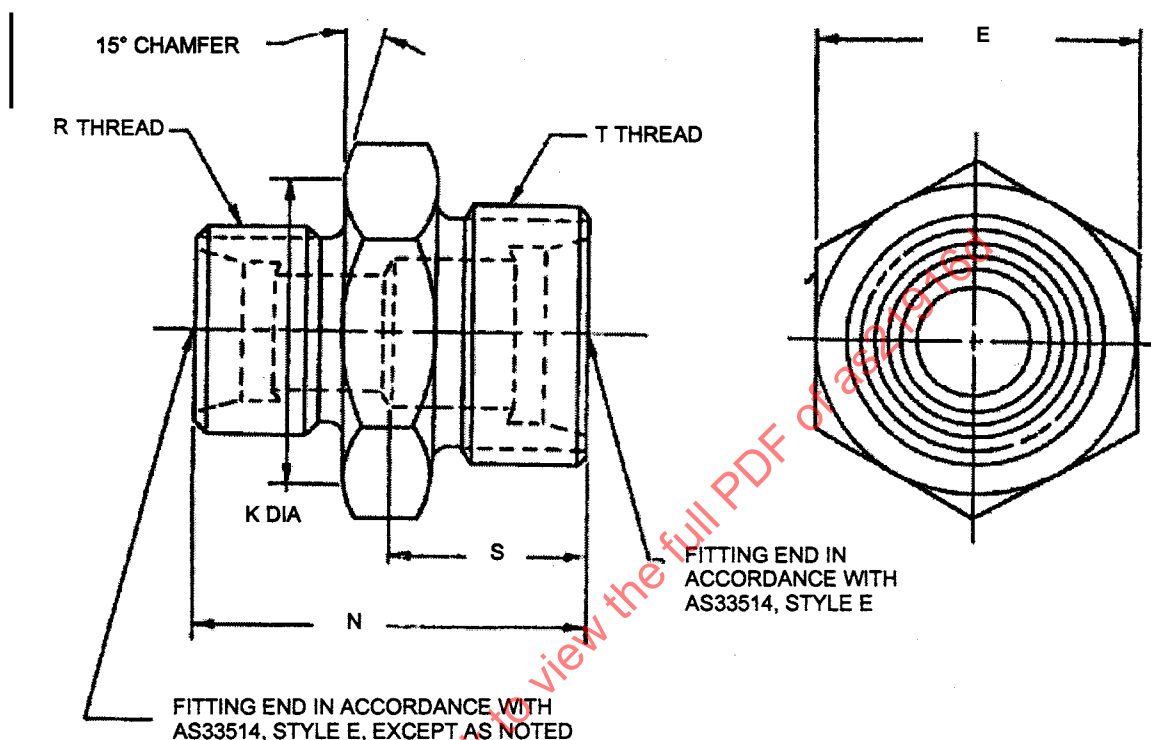
FIGURE 1 - REDUCER, EXTERNAL THREAD, FLARELESS TUBE
