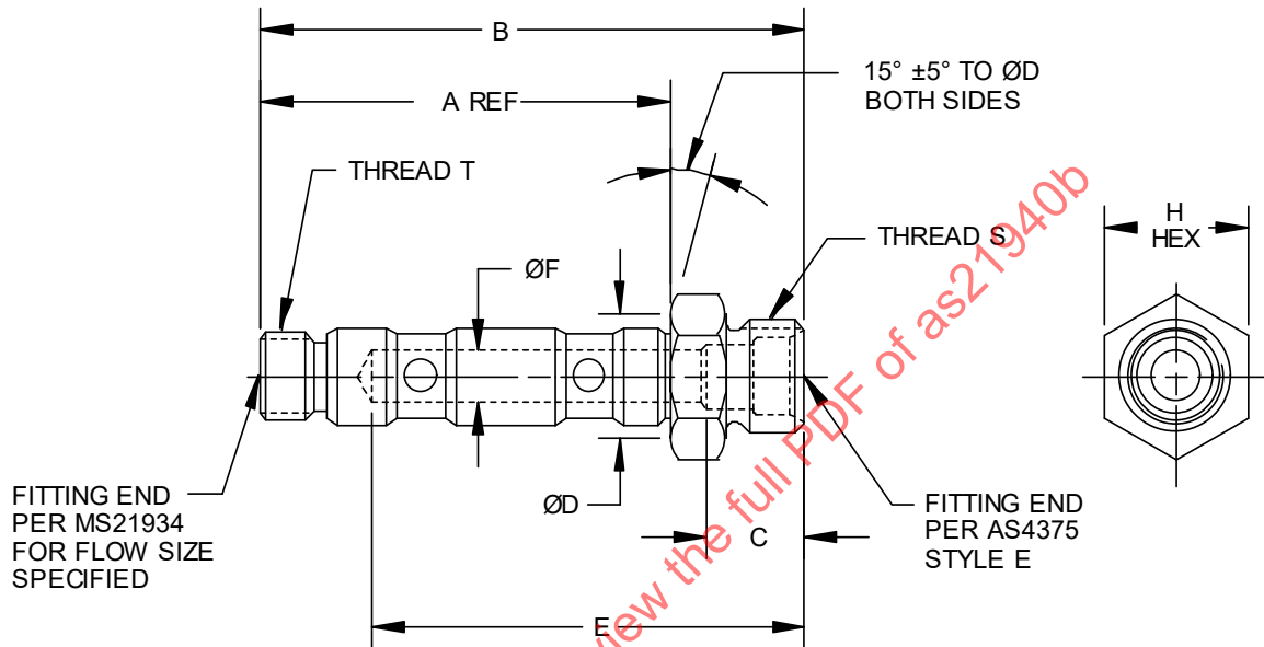
FIGURE 1 - BOLT, CLUSTER FITTING DOUBLE PORT, FLARELESS, DIMENSIONS AND CONFIGURATION
