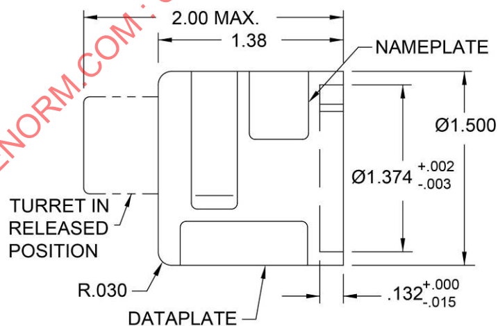
FIGURES 14 - M22520/1-14 TURRET HEAD FOR M39012/03, /35, /36, /38, /40 INNER CONTACTS
