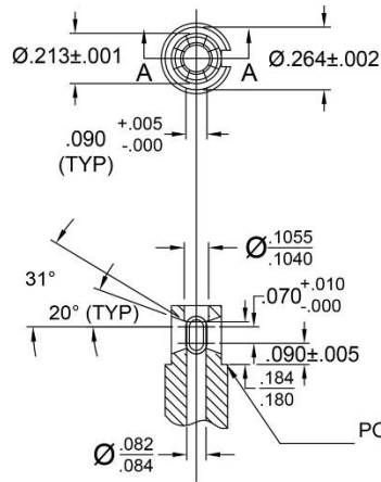
SECTION A-A (WINDOW TYPE) POSITIONER A (RED)
