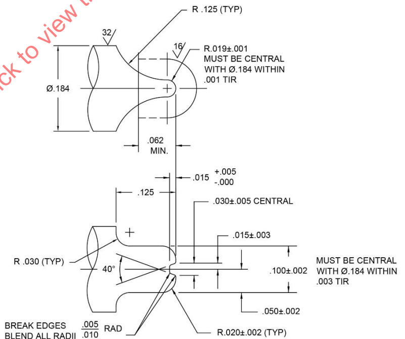
FIGURE 1 - M22520/1-01 TOOL (CONTINUED)
