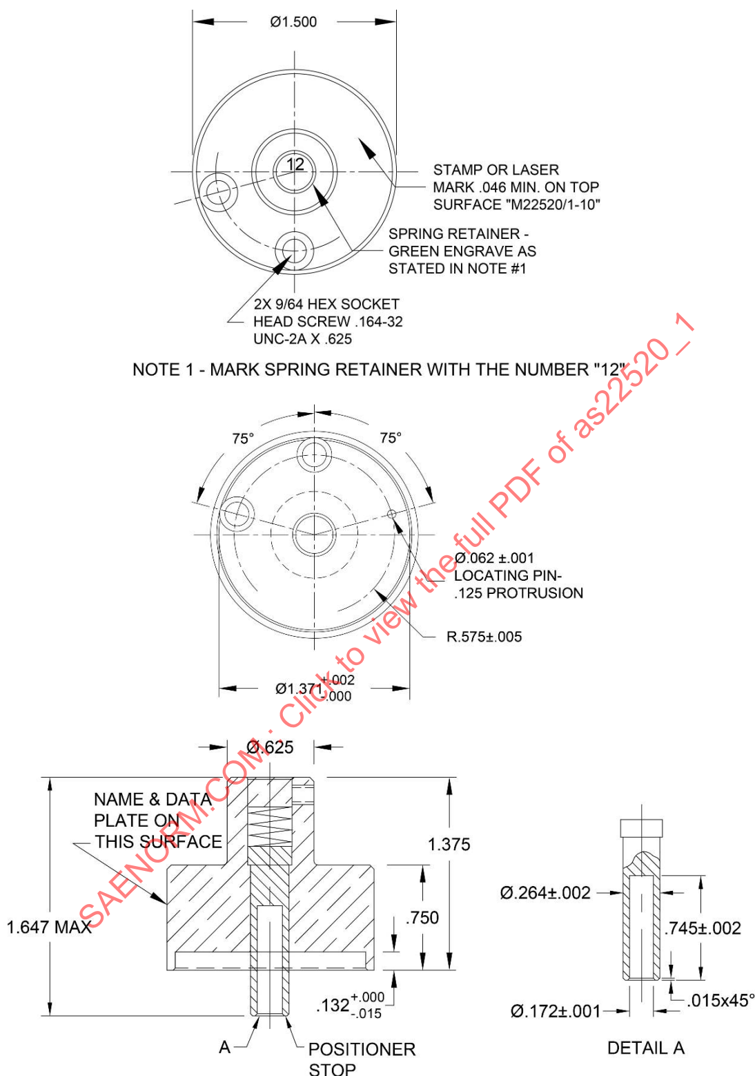
FIGURE 10 - M22520/1-10 POSITIONER FOR M39029/17 CONTACTS
