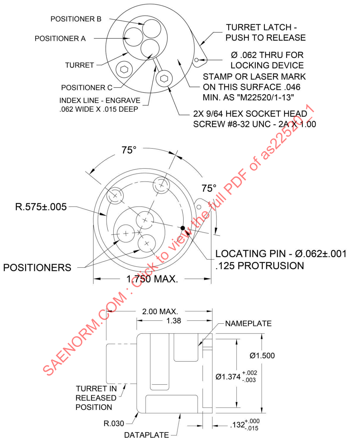
FIGURE 13 - M22520/1-13 TURRET HEAD FOR M39012/01, /02, /05, /39 INNER CONTACTS
