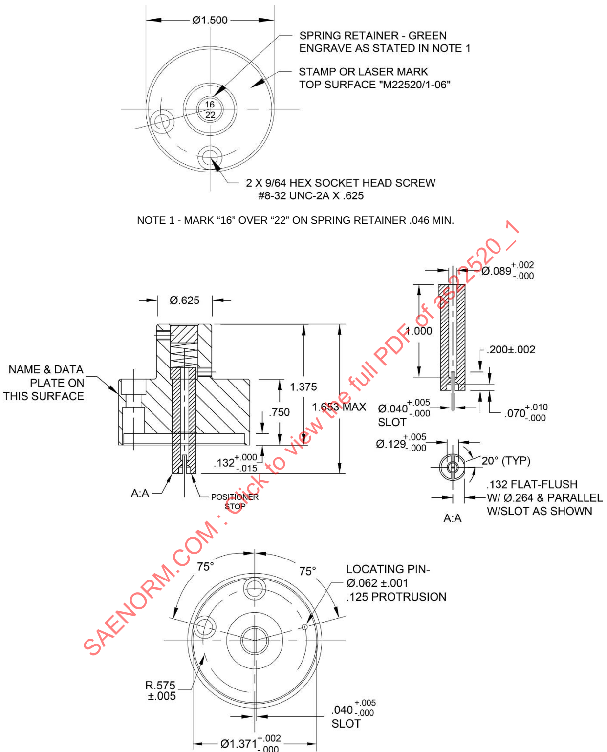
FIGURE 6 - M22520/1-06 POSITIONER FOR OS12814 (TYPE M) CONTACTS
