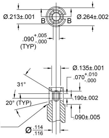
SECTION B-B (WINDOW TYPE) POSITIONER B (BLUE)
