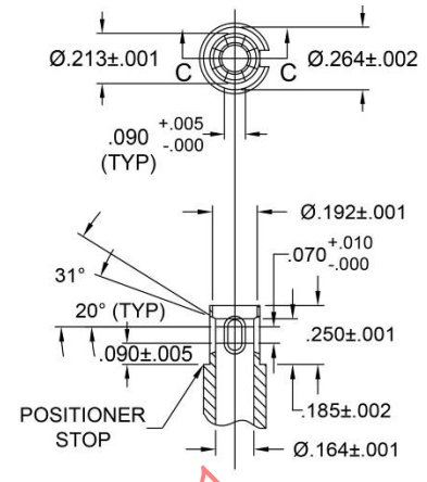
SECTION C-C (WINDOW TYPE) POSITIONER C (YELLOW)
