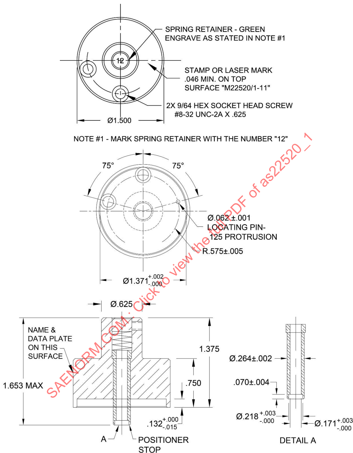
FIGURE 11 - M22520/1-11 POSITIONER FOR M39029/11 AND /12 CONTACTS
