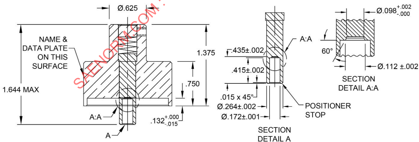
FIGURE 9 - M22520/1-09 POSITIONER FOR M39029/16 AND /18 CONTACTS
