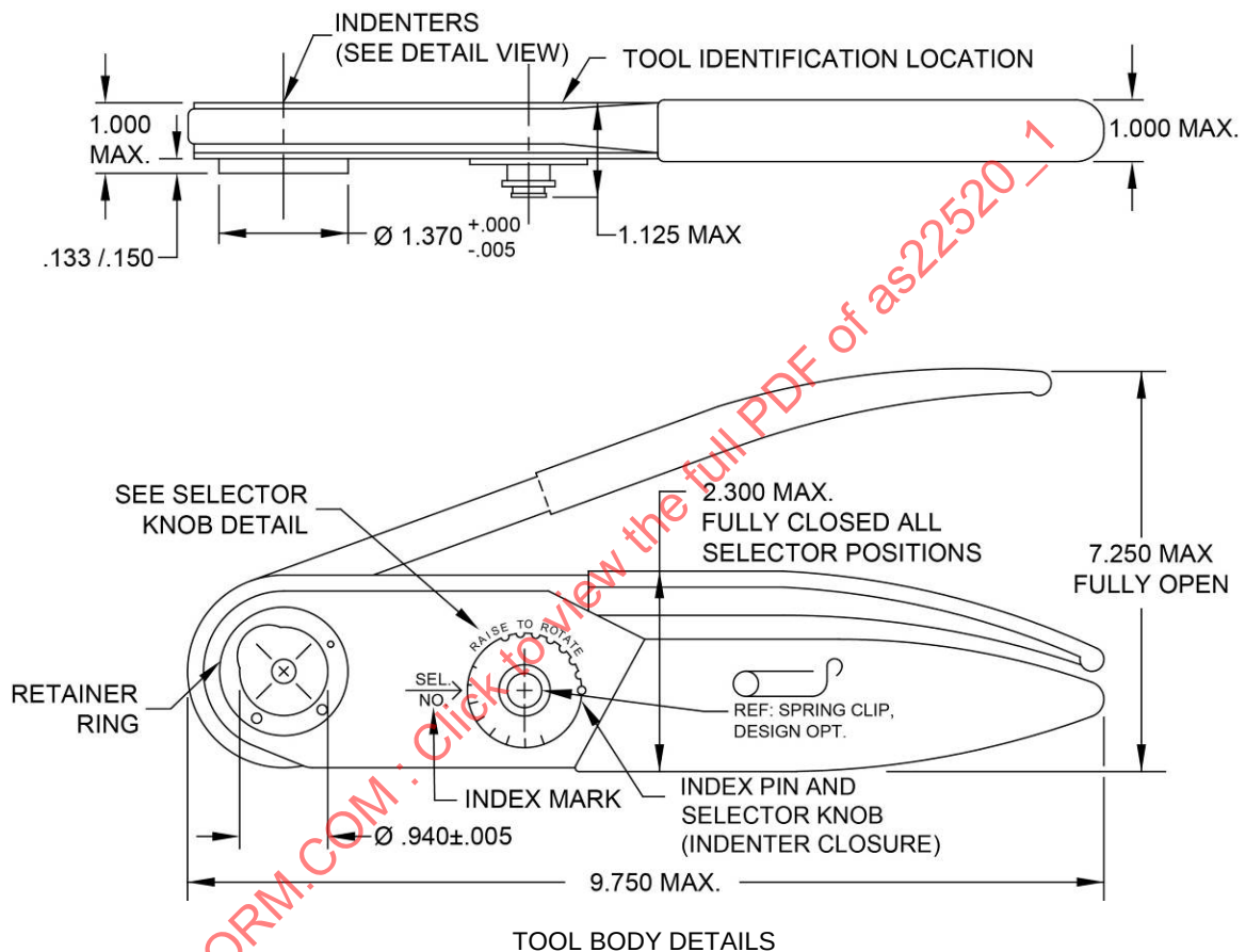
FIGURE 1 - M22520/1-01 TOOL
