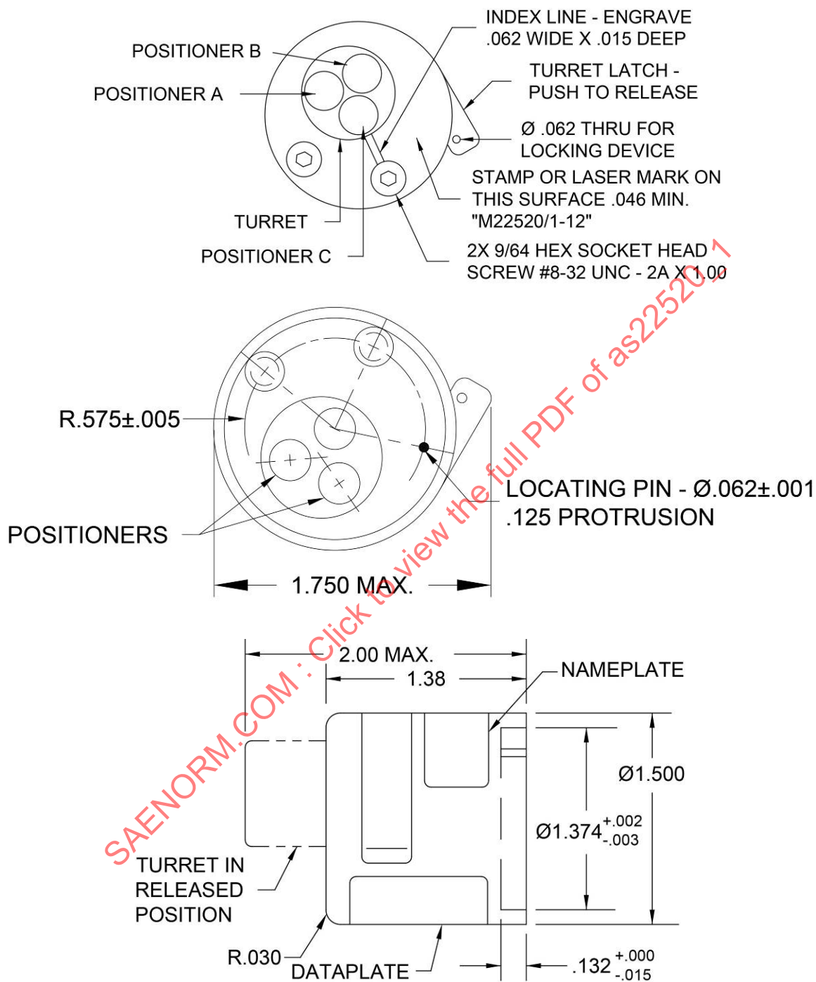
FIGURE 12 - M22520/1-12 TURRET HEAD FOR M39012/16-/20, /26-/30 INNER CONTACTS
