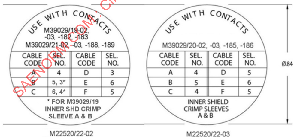
M22520/22-02 AND -04 POSITIONER DATA PLATES
