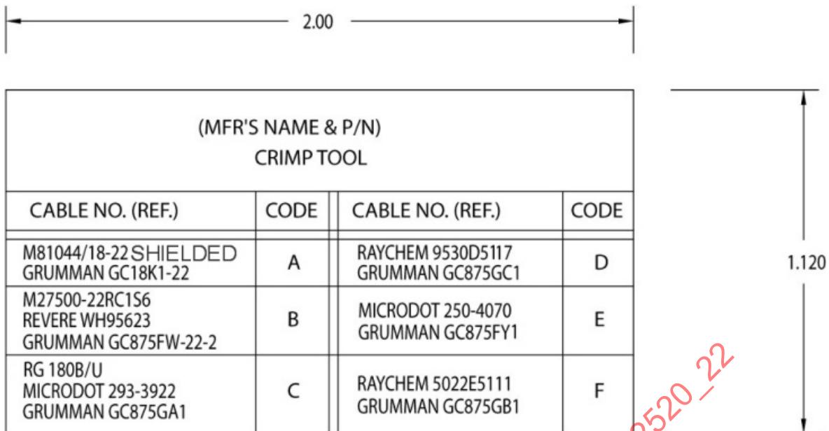
FIGURE 3 - DATA PLATE MARKING REQUIREMENTS (CONTINUED)
