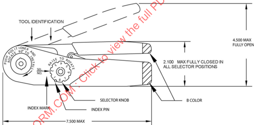
FIGURE 1 - M22520/22-01 TOOL
