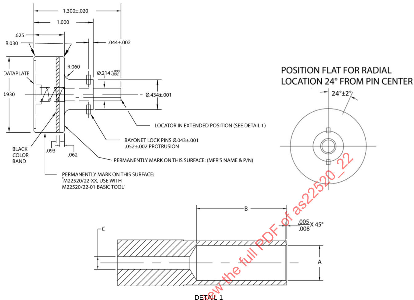
FIGURE 2 - M22520/22 POSITIONER CONSTRUCTION
