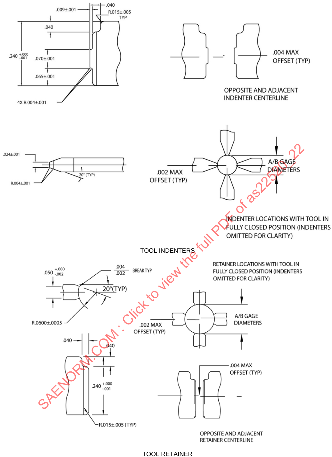
FIGURE 1 - M22520/22-01 TOOL (CONTINUED)
