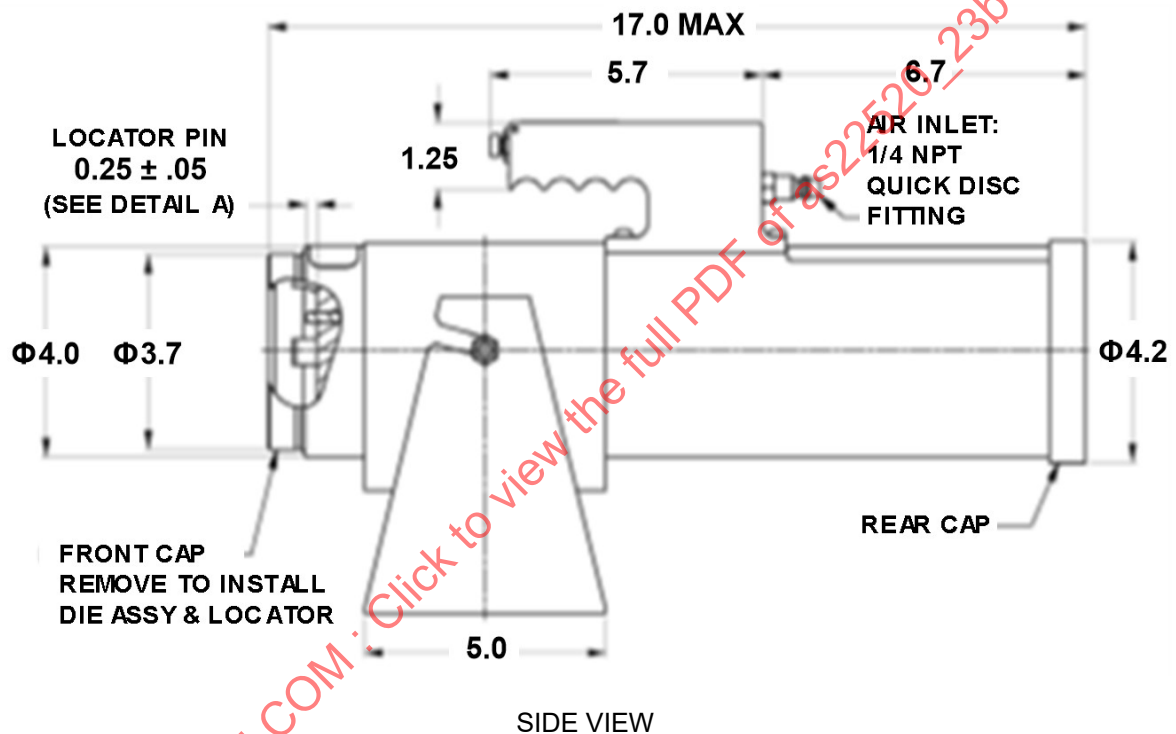
FIGURE 1 - M22520/23-01 BASIC TOOL
