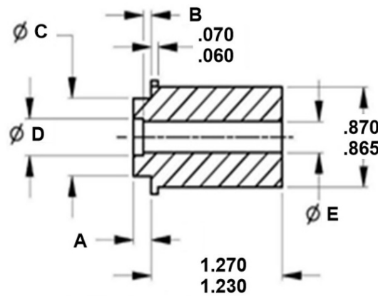
LOCATOR WITH BOSS LOCATES CONTACTS AS39029/29 & AS39029/30 AS39029/44 & AS39029/45
