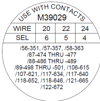
POSITIONER DATA PLATE
