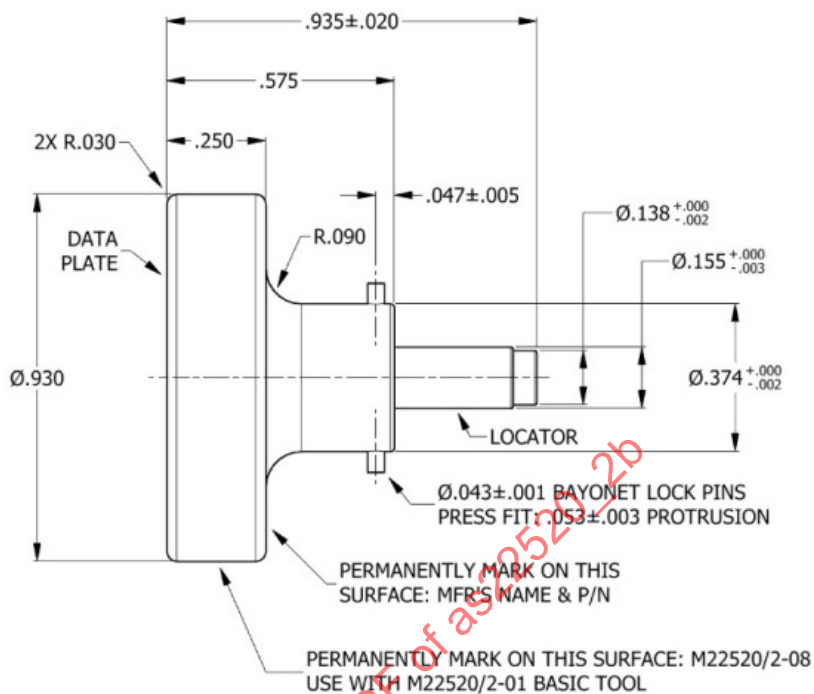
POSITIONER SIDE VIEW
