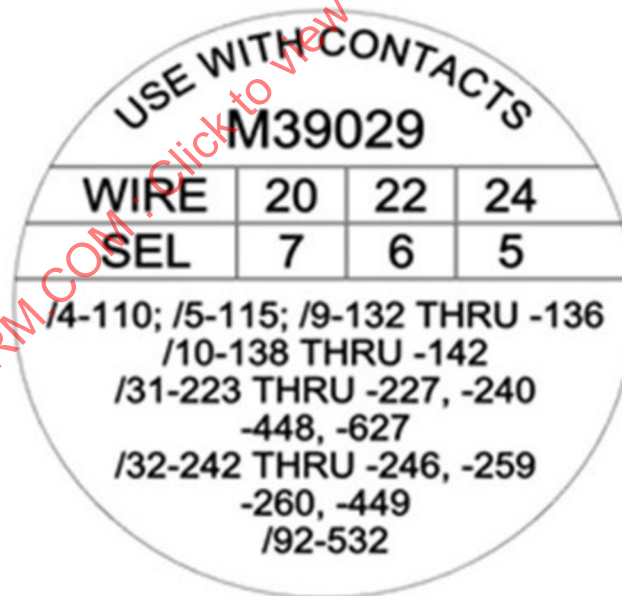
POSITIONER DATA PLATE FIGURE 2 - M22520/2-02 POSITIONER
