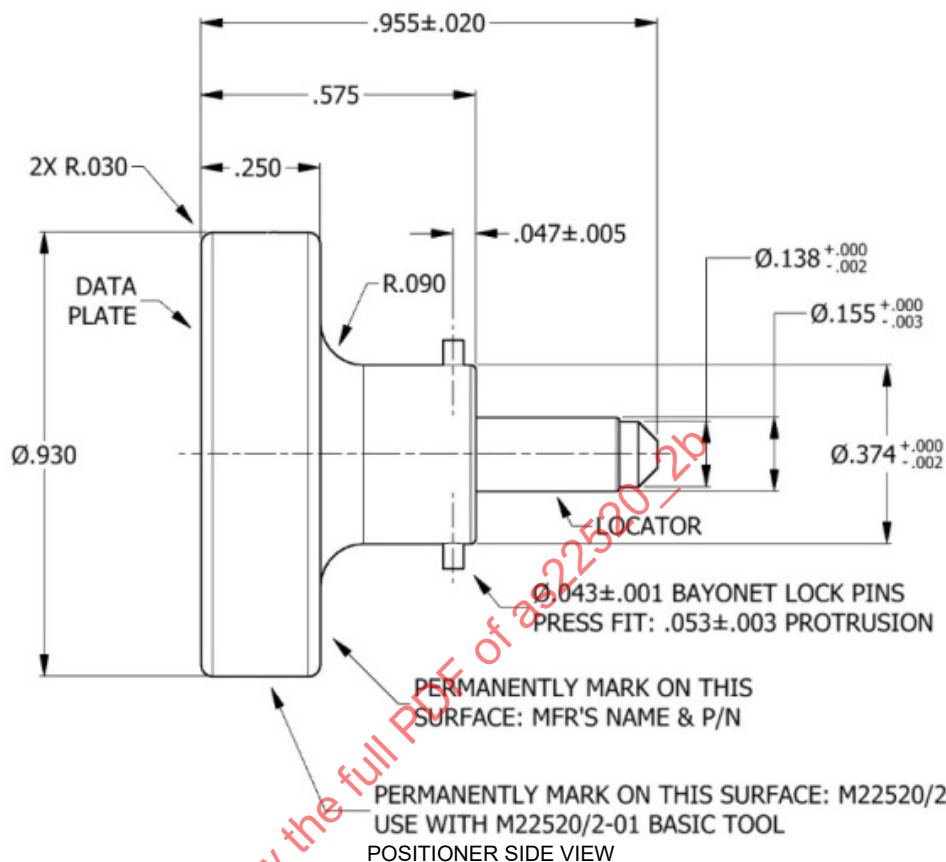
POSITIONER DATA PLATE
