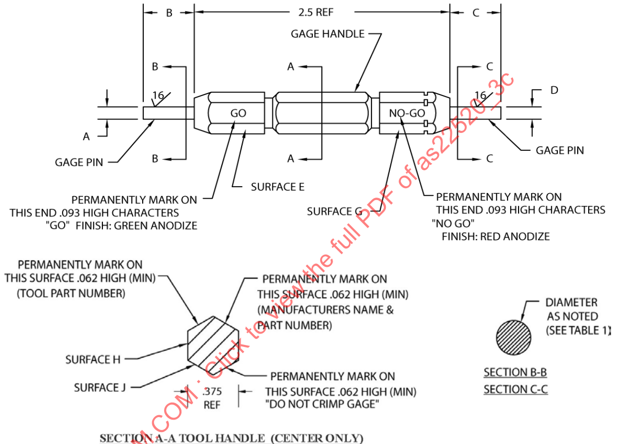
FIGURE 1 - INSPECTION GAGE CONFIGURATION (EXCEPT AS22520/3-17)
