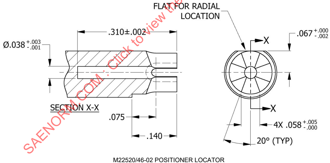
FIGURE 2 - M22520/46-02, 03, -04 , AND -05 POSITIONERS
