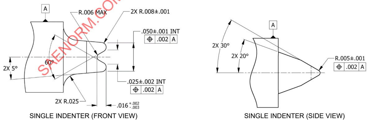
FIGURE 1 - M22520/46-01 TOOL (CONTINUED)
