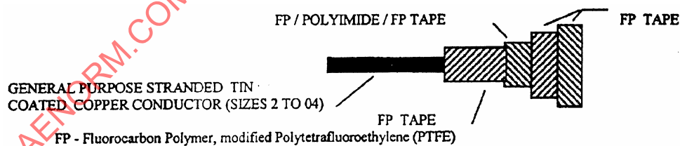
FIGURE 2. GENERAL CONFIGURATION
