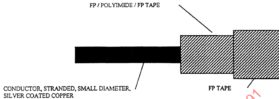
FIGURE 1. GENERAL CONFIGURATION.
