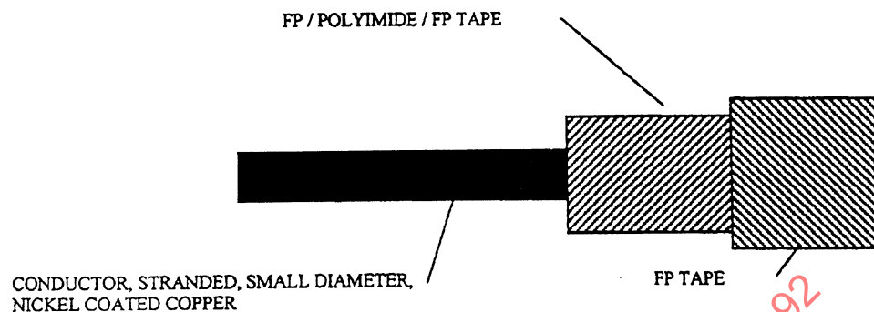
FIGURE 1. GENERAL CONFIGURATION.
