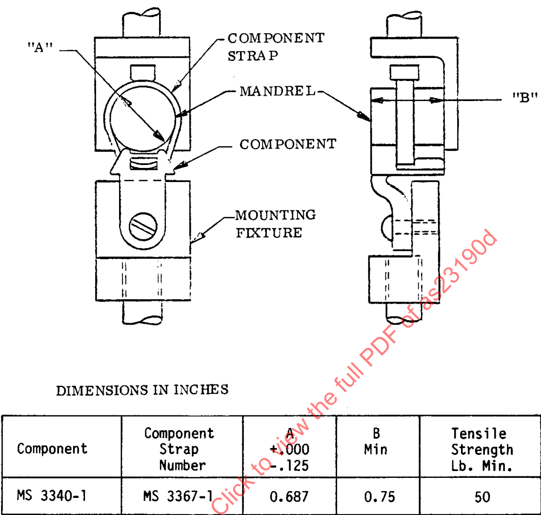
Figure 4 - Tensile test fixture for Type IV bulkhead bracket
