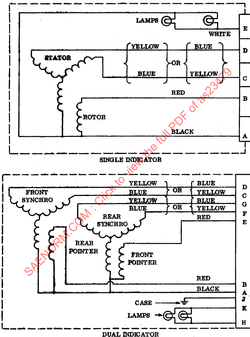
FIGURE 2 - INTERNAL WIRING
