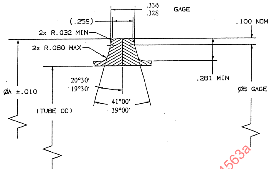
TYPE 2 - MEDIUM WEIGHT SOLID FLANGE PROFILE
