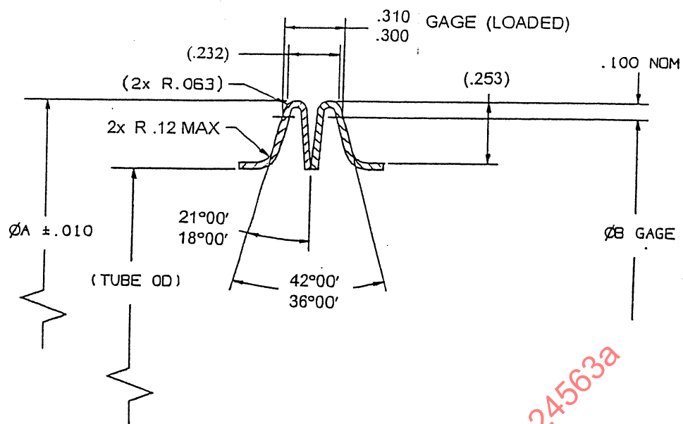
TYPE 4 - NARROW SHEET METAL FLANGE PROFILE
