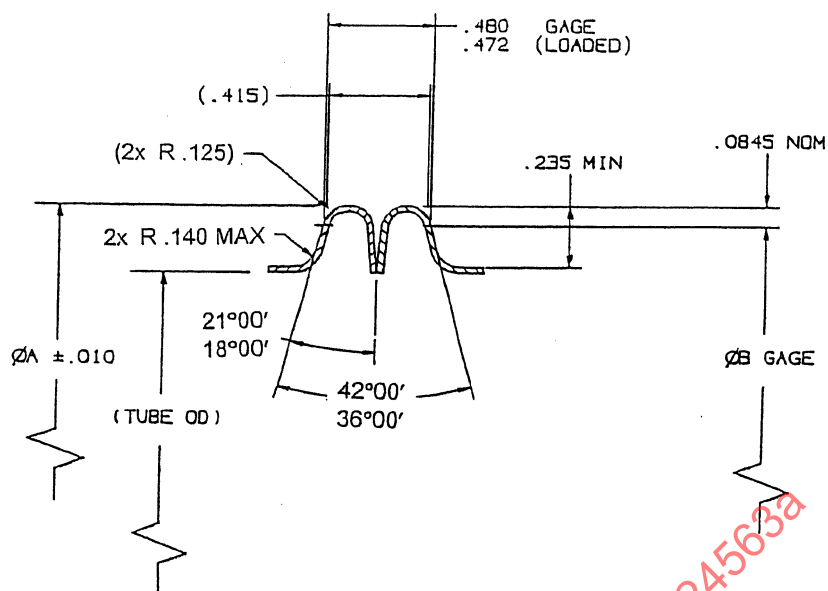
TYPE 5 - WIDE SHEET METAL FLANGE PROFILE
