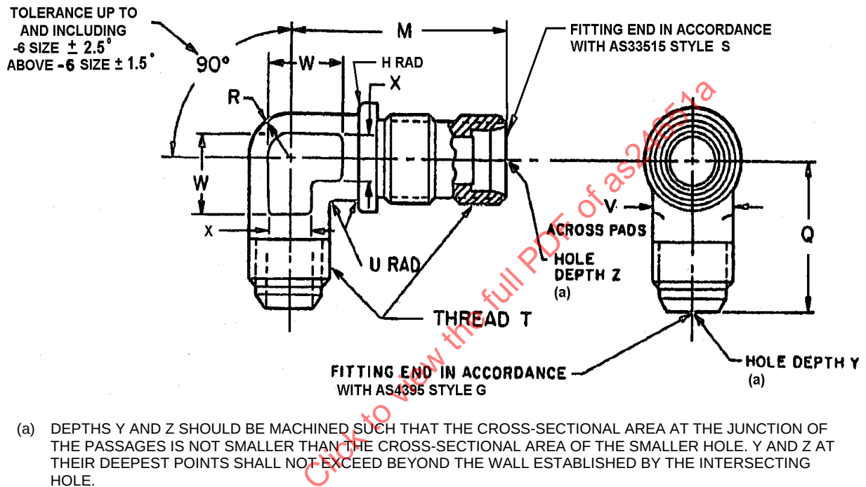
FIGURE 1 ELBOW, TUBE, 90° BULKHEAD, FLARELESS TO FLARED
