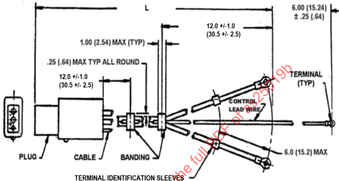
FIGURE 1 - AS25019 CABLE ASSEMBLY
