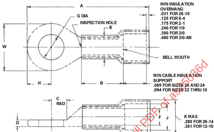
FIGURE 1 – TERMINAL CONSTRUCTION
