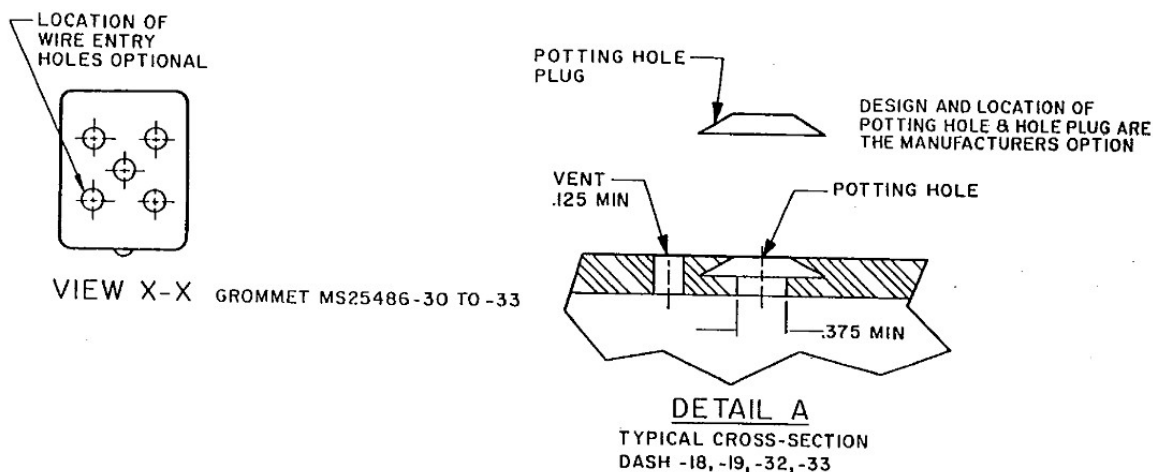
FIGURE 1 (CONTINUED) AS25486 ATTACHABLE PLUG CONFIGURATIONS
