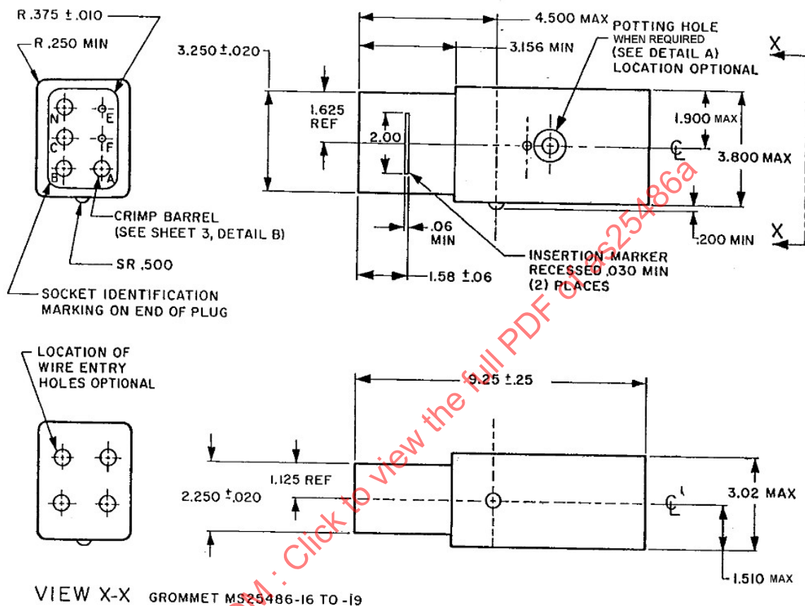
FIGURE 1 – AS25486 ATTACHABLE PLUG CONFIGURATIONS
