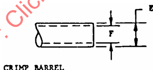
CRIMP BARREL
