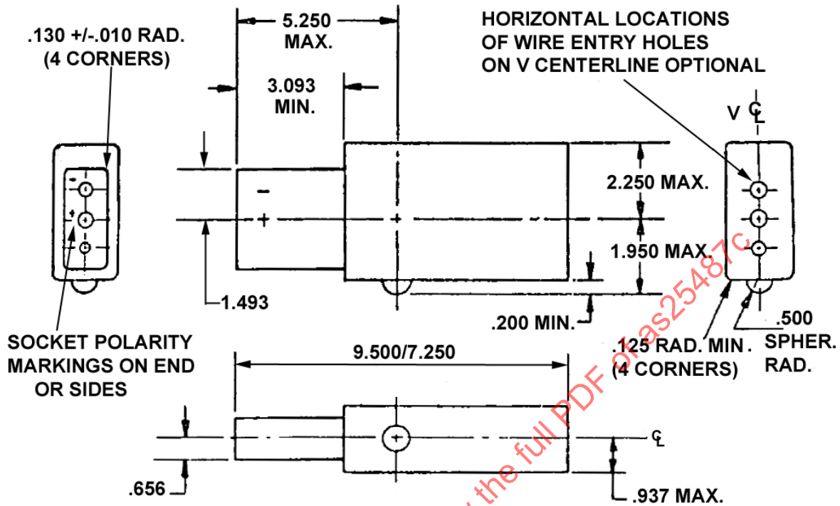
FIGURE 1 - CONNECTOR PLUG
