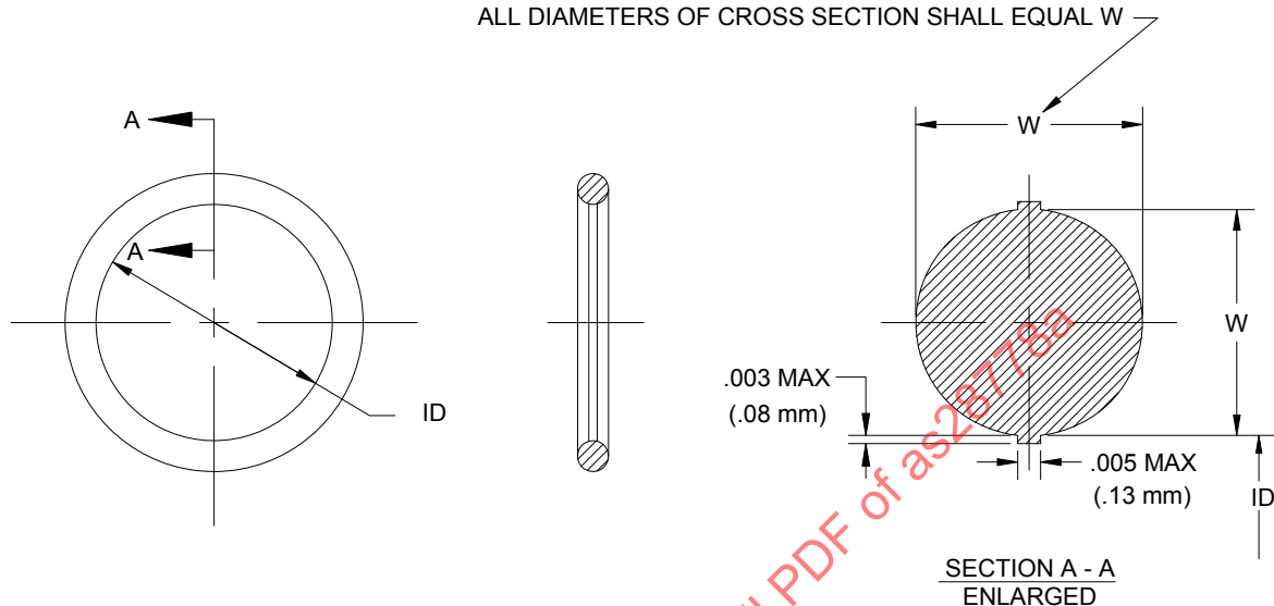
FIGURE 1 - O-RING
