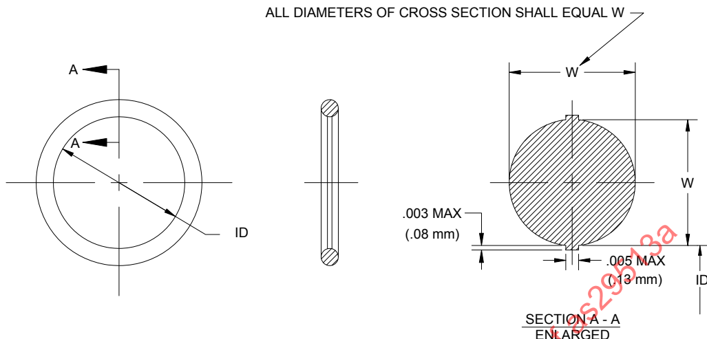
FIGURE 1 - O-RING
