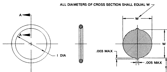
ENLARGED VIEW - SECTION A-A
