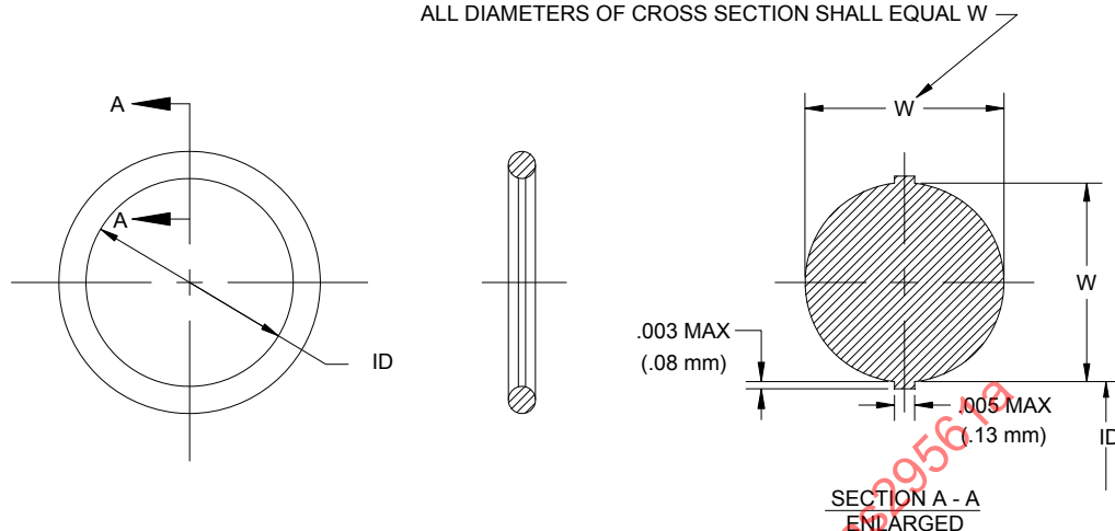
FIGURE 1 - O-RING
