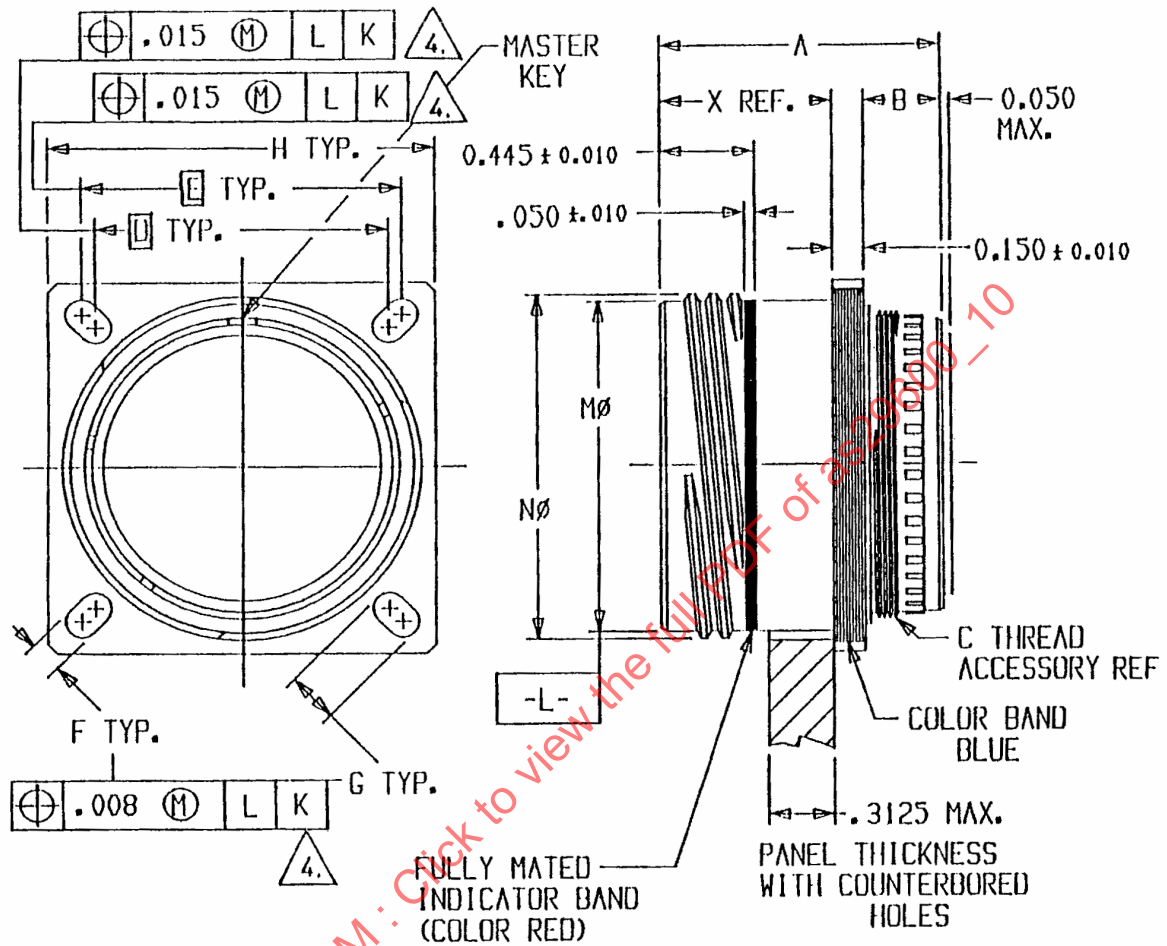
FIGURE 1. M29600/10 COMPOSITE CONNECTOR CONFIGURATION.
