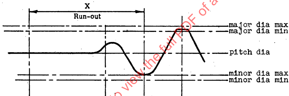
FIGURE 2B. PITCH DIAMETER SHANK FASTENERS
