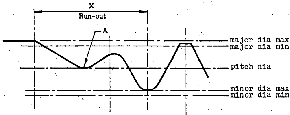
FIGURE 2A. FULL SHANK FASTENERS
