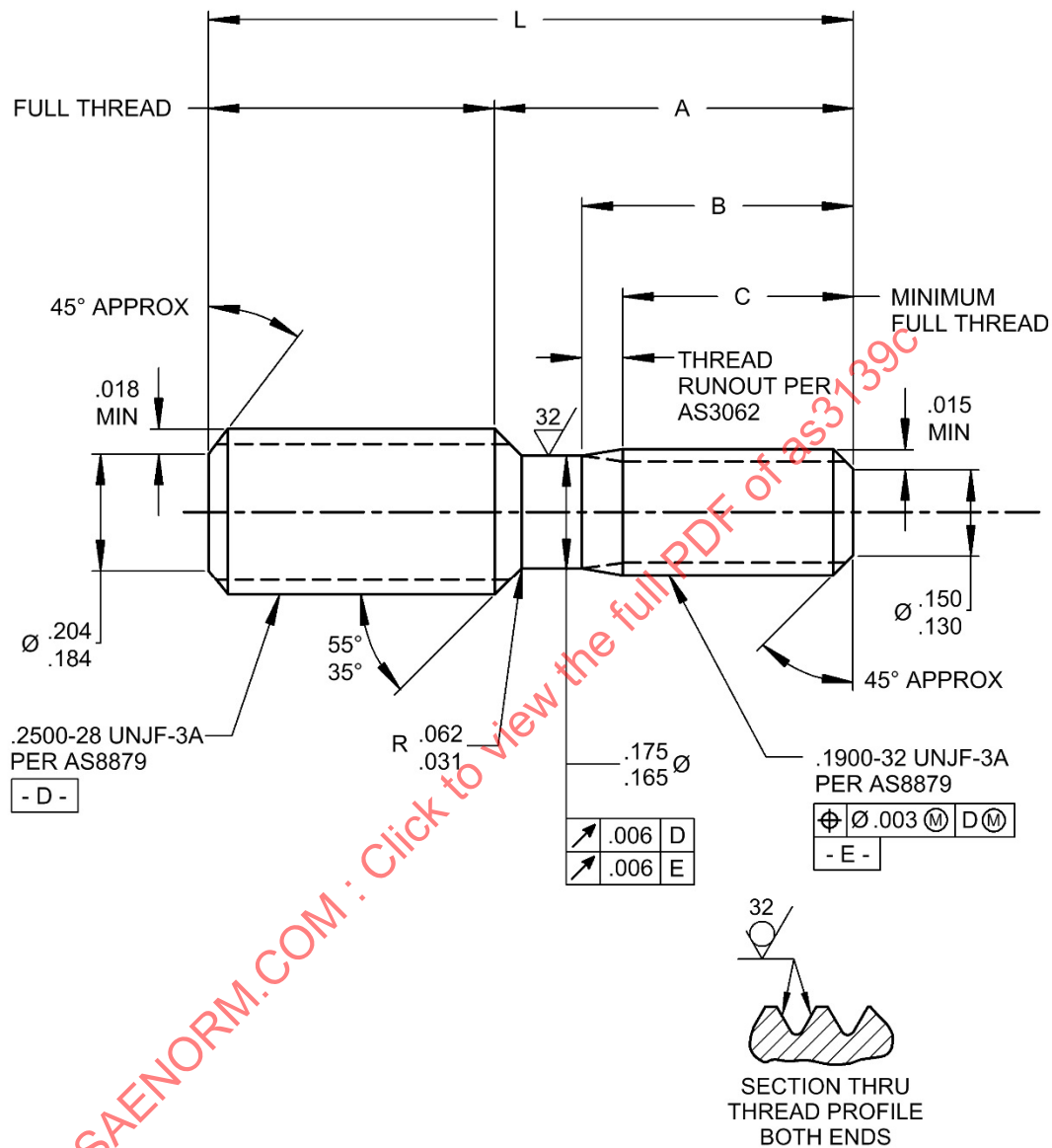
FIGURE 1 - STUD
