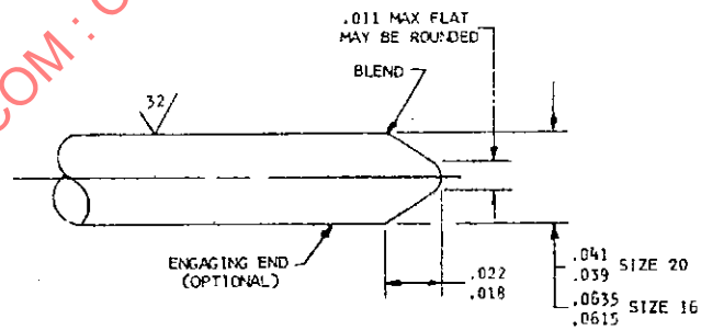
FIGURE 11I CONTACT DETAILS
