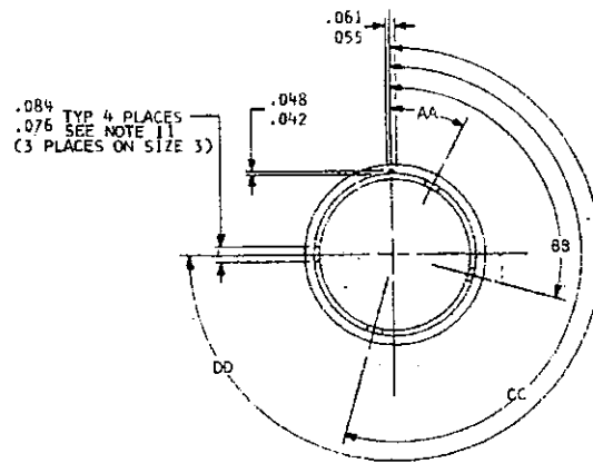
FIGURE 11 KEYWAY POSITIONS
