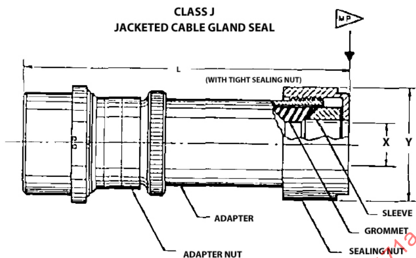
FIGURE 3 – JACKETED CABLE GLAND SEAL
