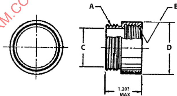
FIGURE 4 – MS3140J-*A, ADAPTER NUT, JACKETED CABLE SEALING
