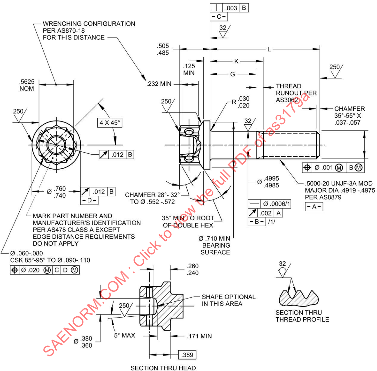
FIGURE 1 - BOLT
