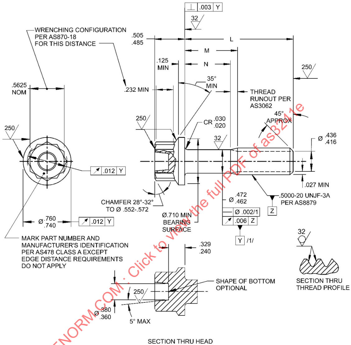
FIGURE 1 - BOLT
