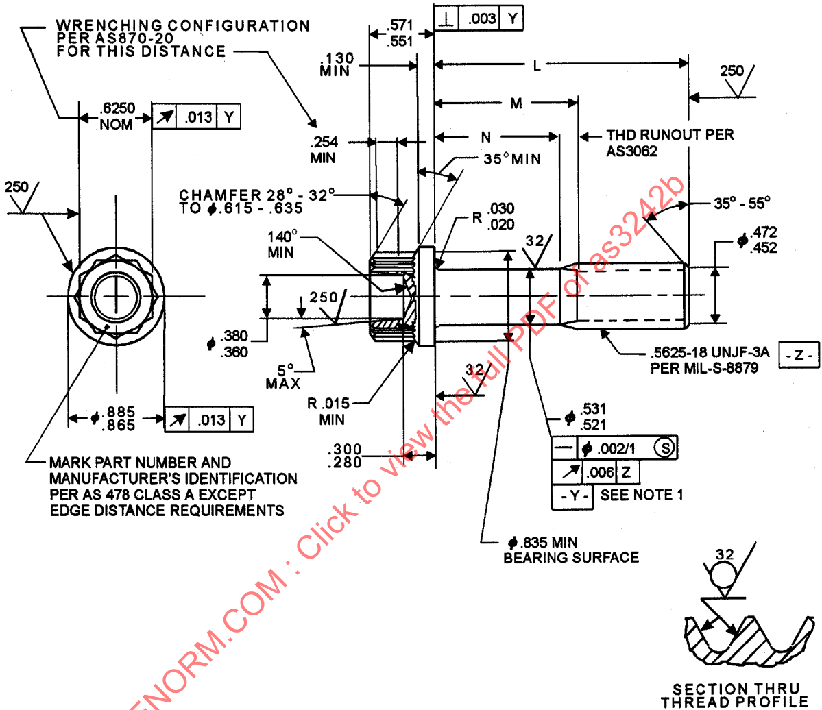
FIGURE 1 - BOLT
